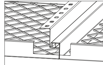
HOOK-ON
